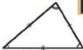
Scalene-triangle
